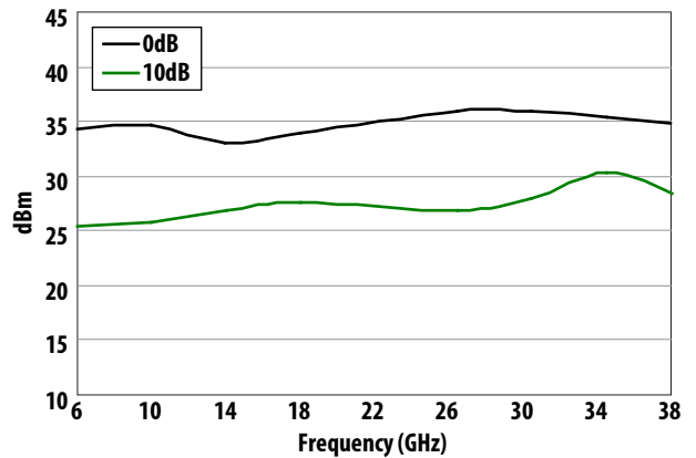
Figure 12. IIP3 vs Attenuation Input Power = 0dBm
